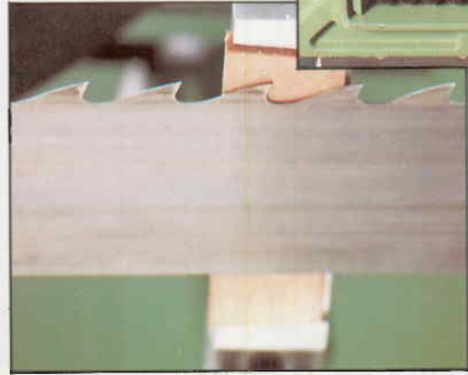
100 mm (4") wide tensioned saw blade. Pressure sawguides for blade stability and cutting accuracy.
