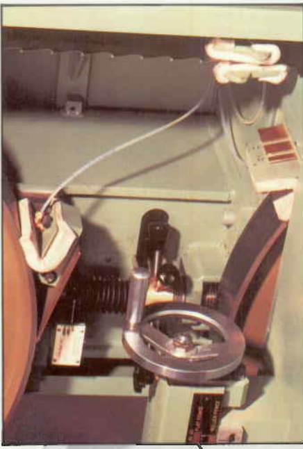
Saw wheels cleaned by scrapers and lubricated pads. Blade cleaned by spring loaded pads.
